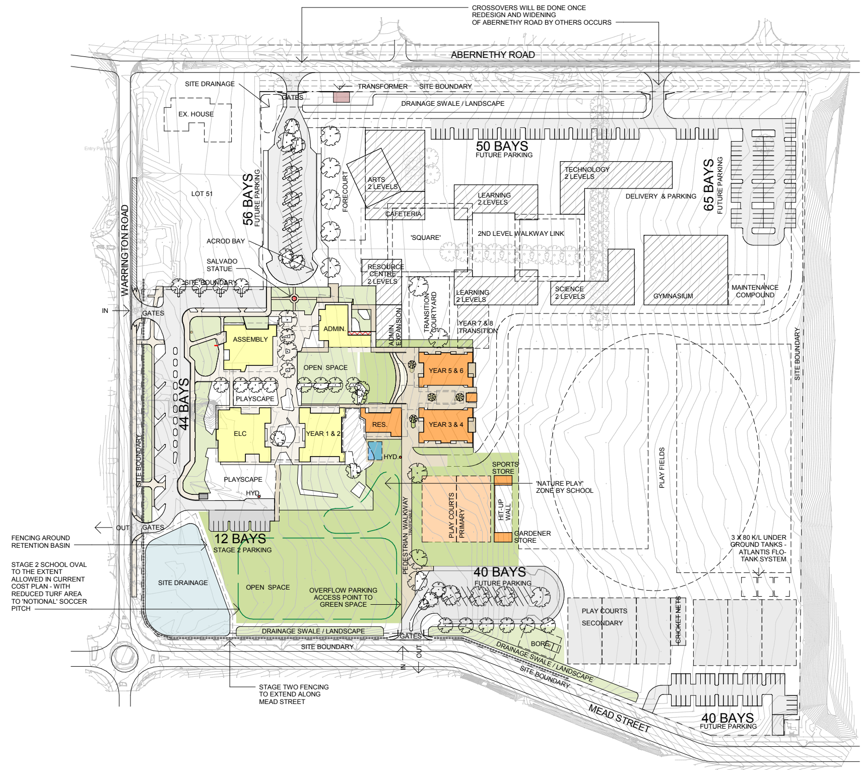
OVERALL MASTERPLAN SCALE: 1: 1000 @ A1
